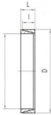
基本尺寸和参数 Basic dimensions and parameters of the locking assemblies, type Z1
