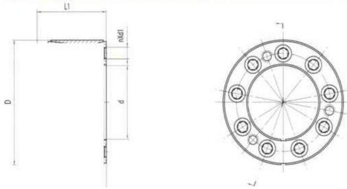
基本尺寸和参数 Basic dimensions and parameters of the locking assemblies, type Z4
