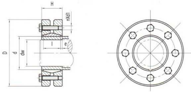
基本尺寸和参数 Basic dimensions and parameters of the locking assemblies,type Z7A
